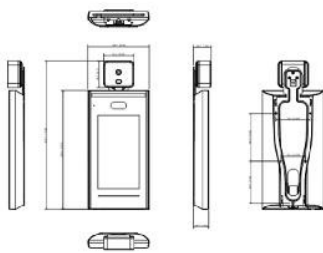
Dimensions (mm[inch])
